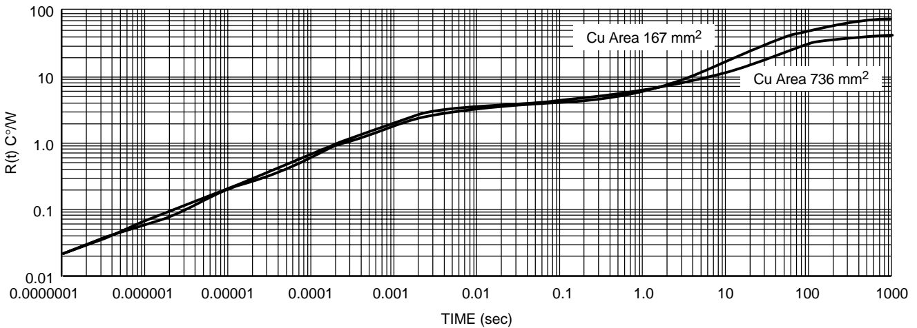
Figure 9. Single-Pulse Heating Curves, D 2 PAK 5-Lead
